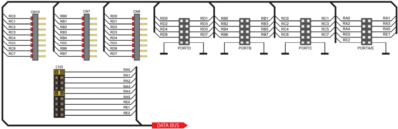
Figure 2-14: Input/Output Group
