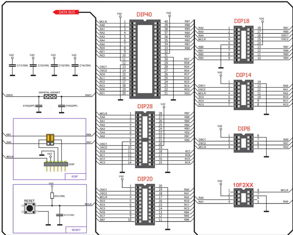
Figure 2-2: MCU System
