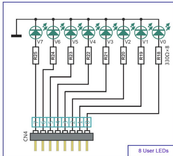
Figure 2-5: 8 LEDs
