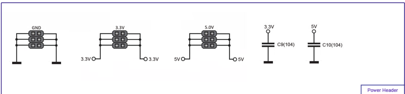
Figure 2-15: Power Supply Header for DIY
