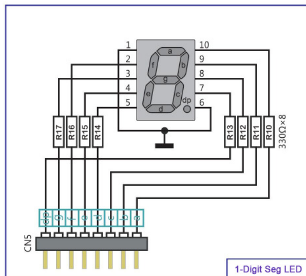
Figure 2-4: 1-Digit SegLED Display Module
